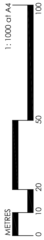
19.0m Semi - On-Road Swept Turning Paths
